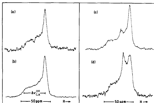
Fig.3. 36.4 MHz ^{31}\text{P} NMR spectra at 37^\circ\text{C} in the presence of broad band proton decoupling. (a) Normal erythrocyte ghosts; (b) liposomes composed of lipids extracted from erythrocyte ghosts; (c) ether extracted ghosts; (d) liposomes composed of lipids from ether extracted erythrocyte ghosts. All preparations contained 25 mM Tris-HAc (pH 7.2).
