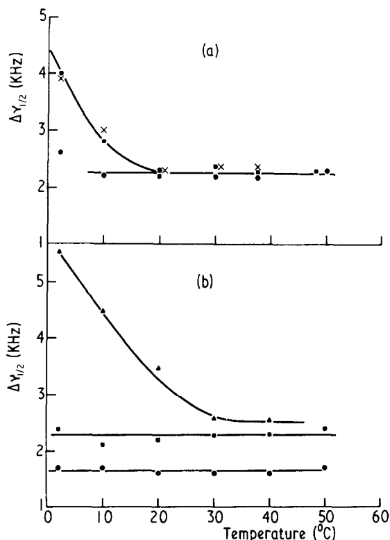
Fig.1. Temperature dependence of \Delta\gamma_{1/2} of the 129 MHz 31 P NMR spectra obtained from erythrocytes and derived liposomes (a) ● - erythrocyte ghosts; ■ - erythrocyte ghosts after ether extraction; X - pronase digested ether extracted ghosts (b) ● - liposomes composed of total lipids from erythrocyte ghosts; ■ - liposomes composed of total lipids from ether extracted ghosts; ▲ - partially hydrated (14% by wt) total lipids from ether extracted ghosts. All fully hydrated ghost and derived liposome preparations contain 25 mM Tris-HAc (pH 7.2).
