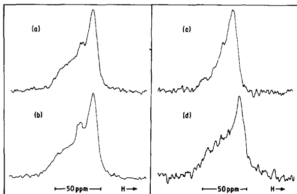
Fig.2. 129 MHz ^{31}\text{P} NMR spectra at 37^\circ\text{C} in the absence of proton decoupling: (a) normal erythrocyte ghosts; (b) erythrocyte ghosts after ether extraction; (c) liposomes (completely hydrated) of lipids extracted from the ether extracted ghosts; (d) partially hydrated (14% by wt) lipids from ether extracted ghosts. All fully hydrated ghost and liposome preparations contain 25 mM Tris-HAc (pH 7.2).
